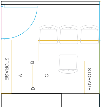
CABIN 02
